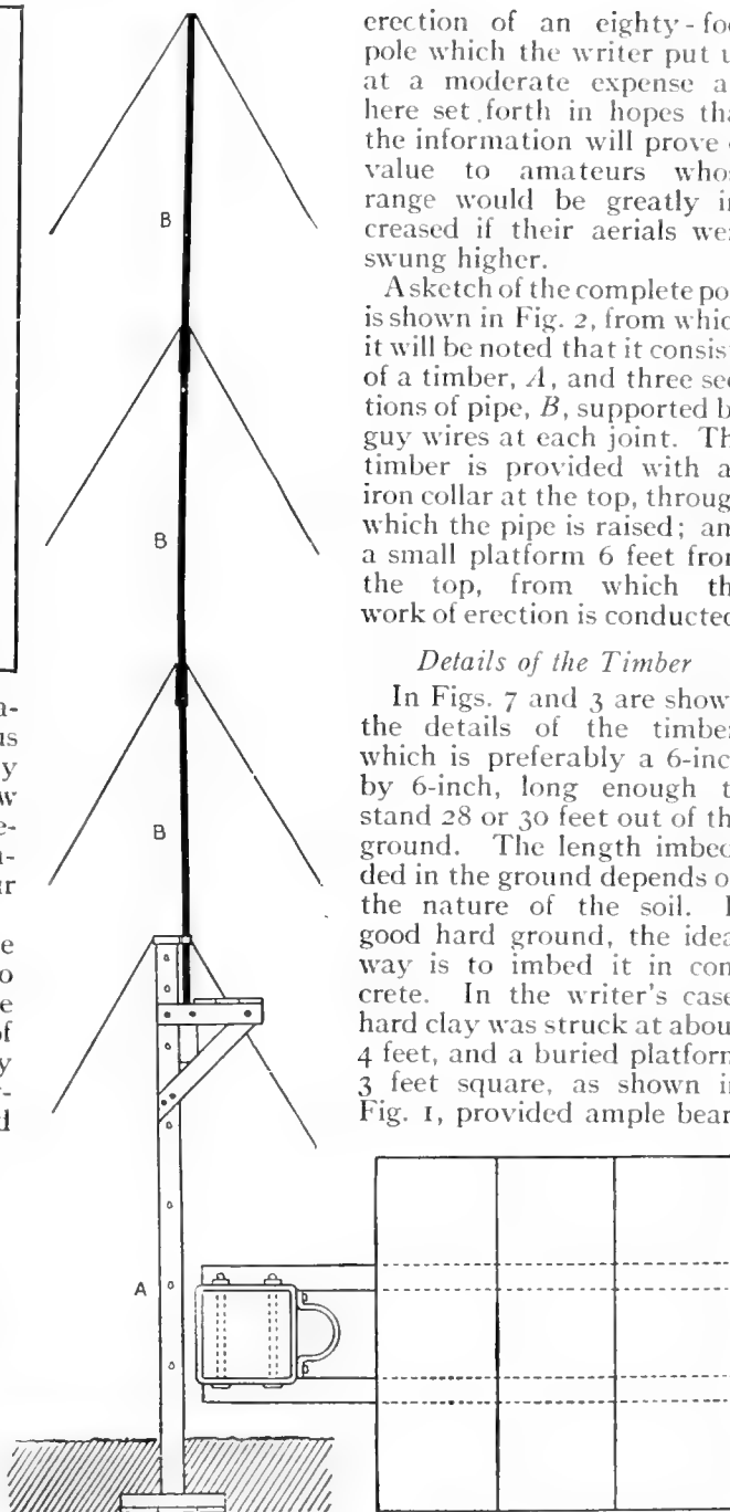
Fig. 2. The Mast Complete
